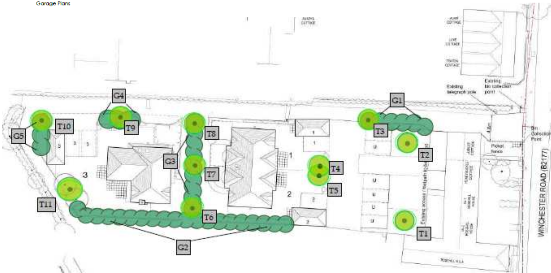
Garage Plans
